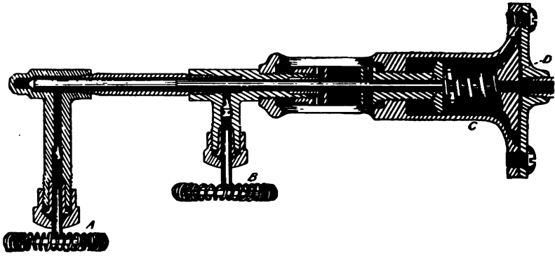
FIG. 312.—Fuel Feed Regulator of a Steam Carriage Burner, intended for Use with "Torch" Burner Kindler or Auxiliary Vaporizer. A is the hand wheel and needle valve regulating the feed to the main burner; B, the hand wheel and valve for operating the torch; C, the spring and header attached to the main valve rod; D, the diaphragm against which steam bears, regulating the main valve according to pressure. The liquid gasoline is admitted at a port on the left-hand extremity of the regulator tube, near the end of the needle valve on the main rod.
